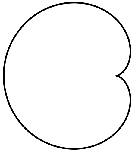
Cardioid
