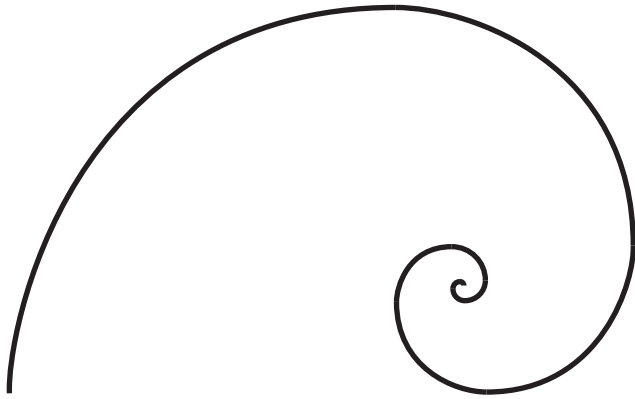
Logarithmic spiral
