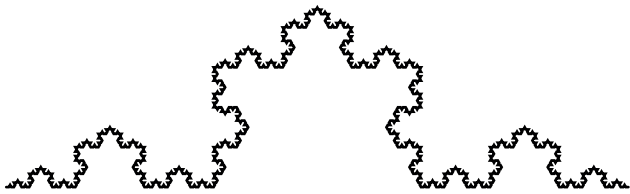
Koch curve
